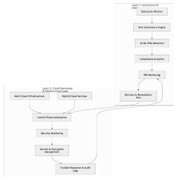
Intelligent Risk & Compliance Orchestration – Double Layer Flowchart
